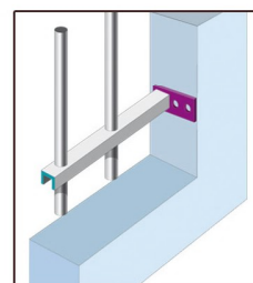
T/5 platine 40x100x5
