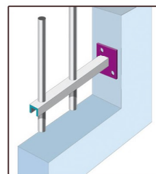
T/3 platine 80x80x5
